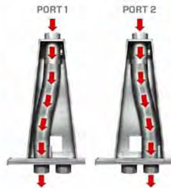
This diagram shows the isolation of the off leg to eliminate material cross contamination
